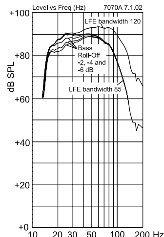
Figure 10. The free field frequency response of 7070A and 7071A subwoofers at different Bass Roll-Off settings.
